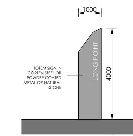
TOTEM SIGN - PROPOSED ELEVATION SCALE 1:100 @ A1
