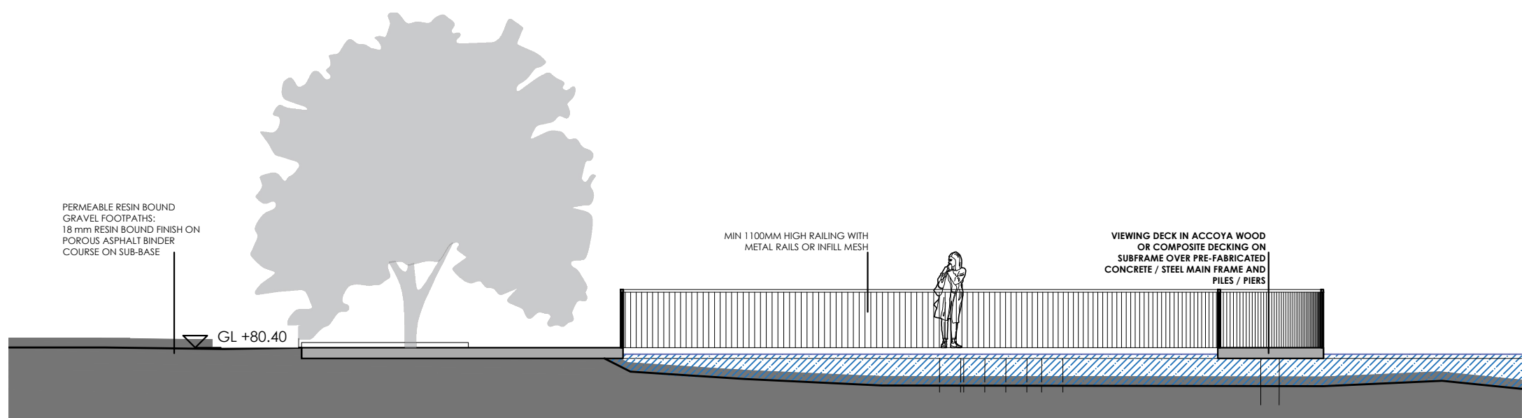
CRANNÓG VIEWPOINT - PROPOSED SECTION D-D SCALE 1:100 @ A1
