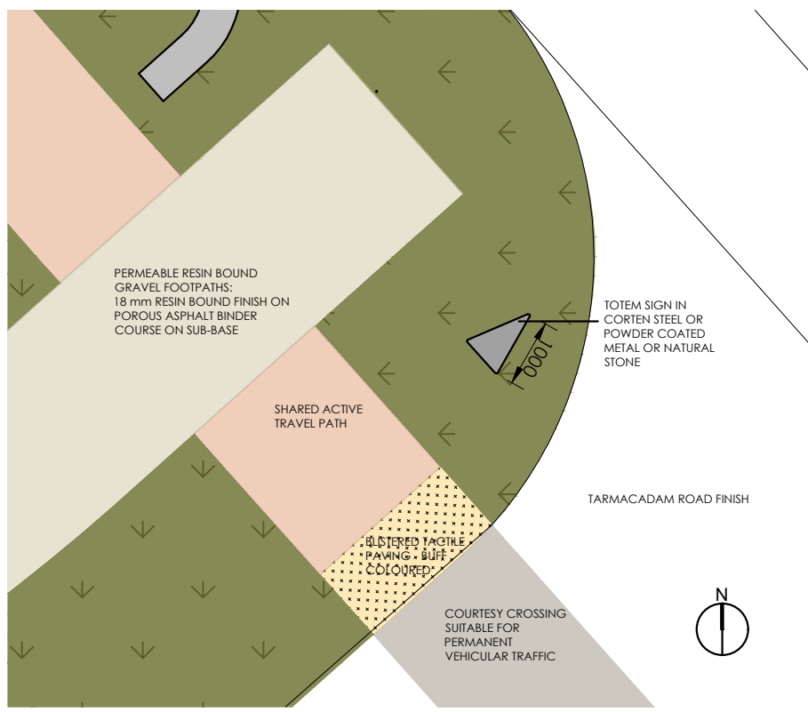
TOTEM SIGN - PROPOSED PLAN SCALE 1:100 @ A1
